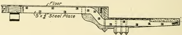
Fig. 7. Platform Knee
